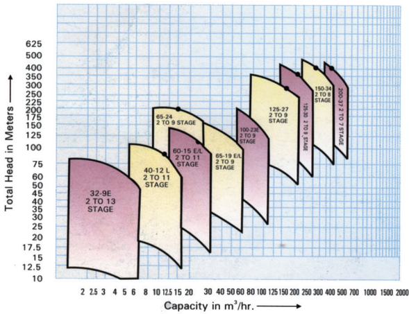
Family Curves of multistage pumps at 1750 rpm - 60 Hz
