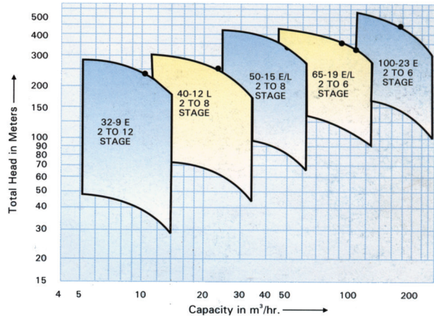
Family Curves of multistage pumps at 3500 rpm - 60 Hz
